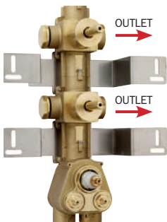
THERMOSTATIC Z030201000 2 OUTLETS
