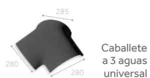
Caballete universal
